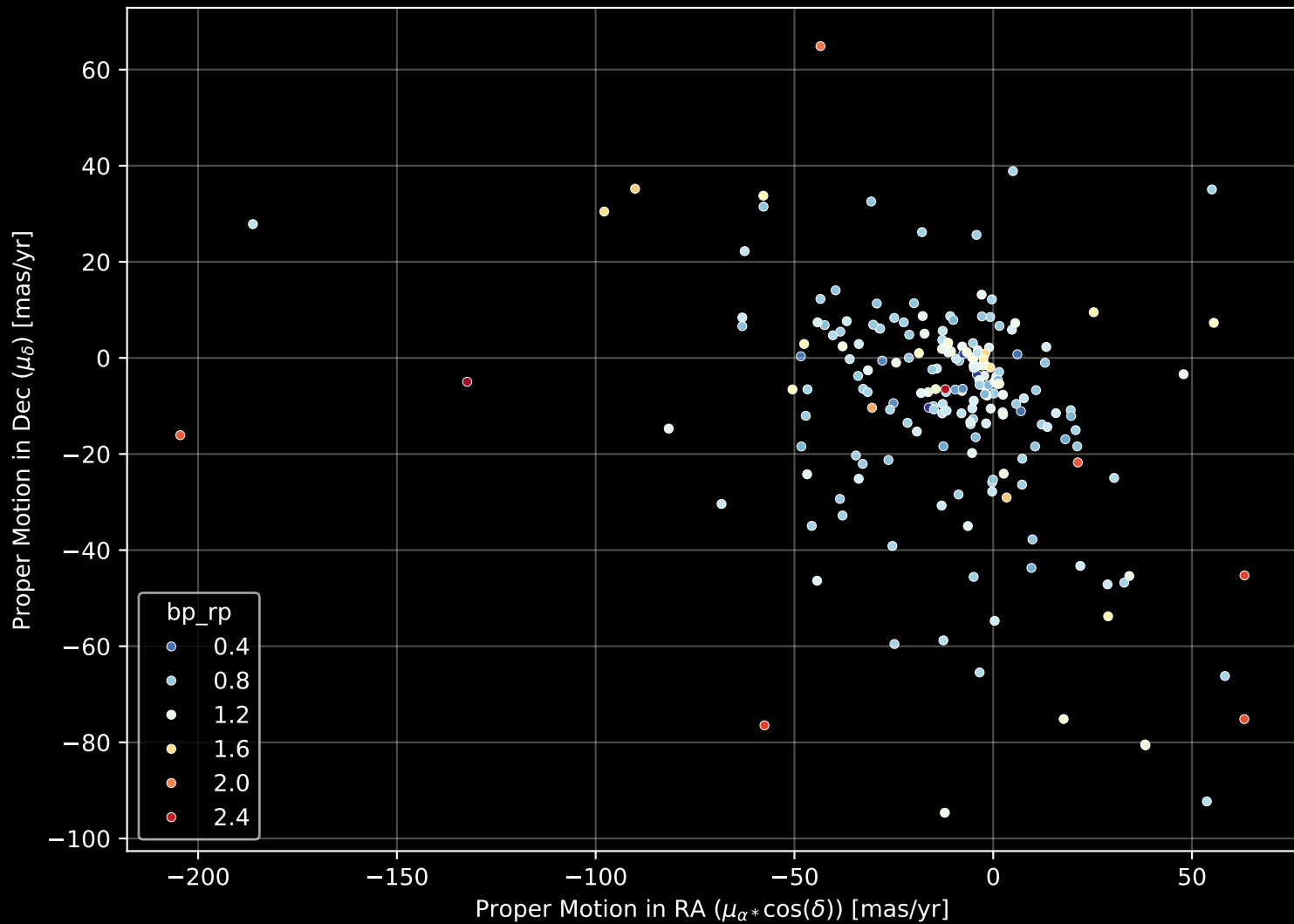
APOGEE DR17 Field: [237+44_MGA] Proper Motion Diagram (n= 204)
