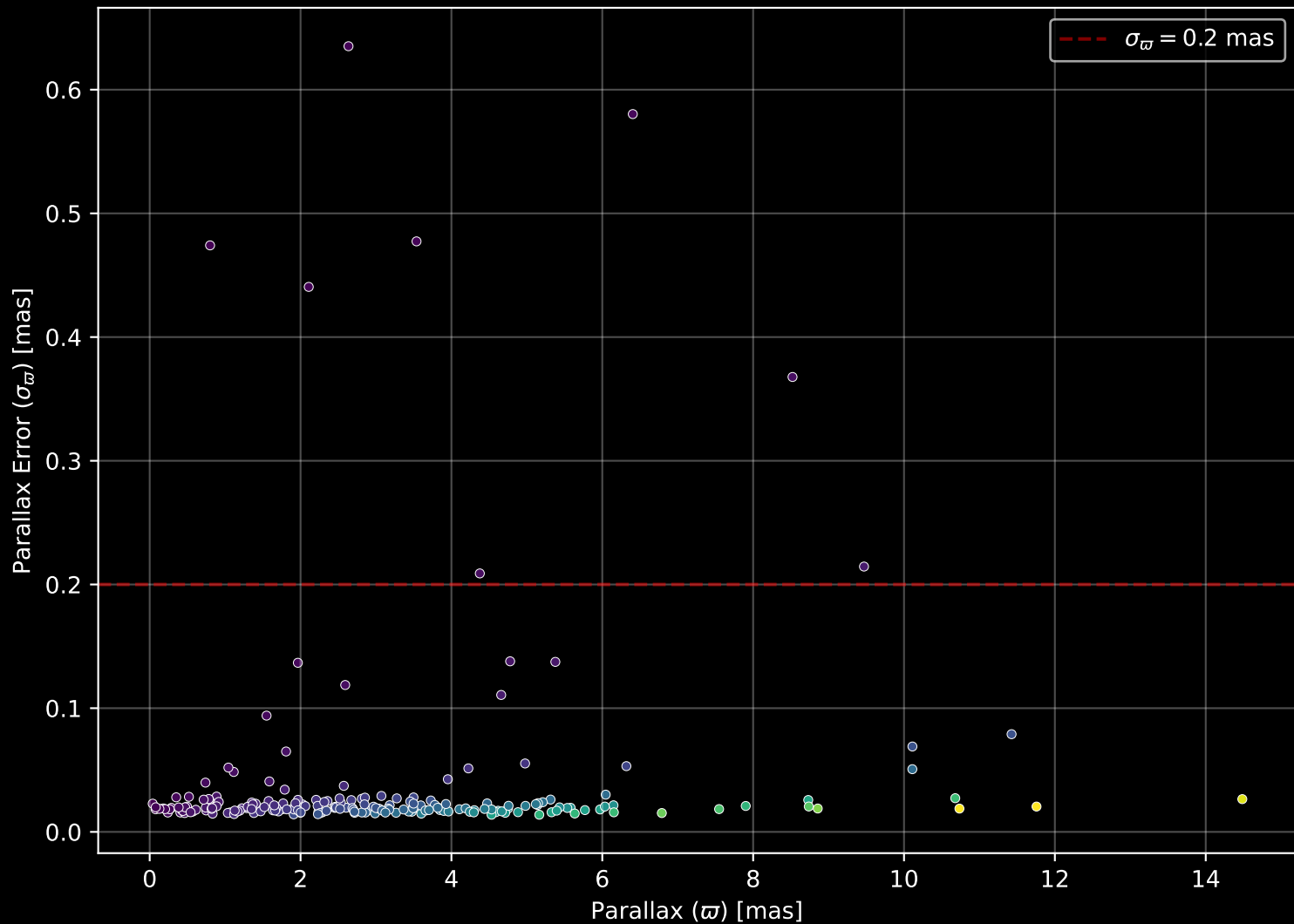
APOGEE DR17 Field: [237+44_MGA] Parallax Quality (n= 204)
