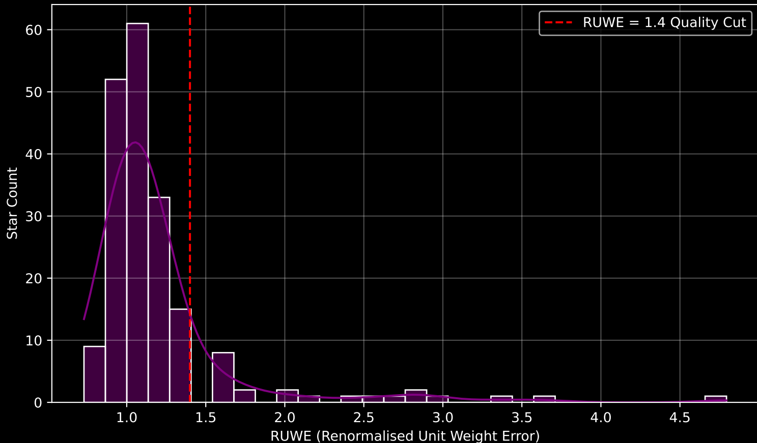
GAPOGEE DR17 Field [237+44_MGA] RUWE Distribution (n= 192)
