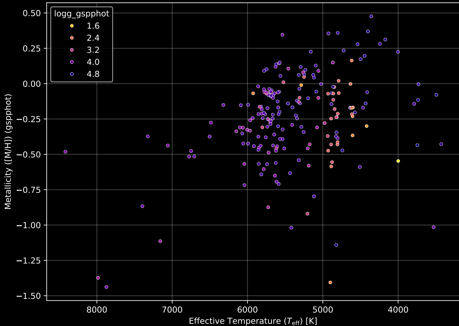
APOGEE DR17 Field: [237+44_MGA] Stellar Population Parameters (n= 204)
