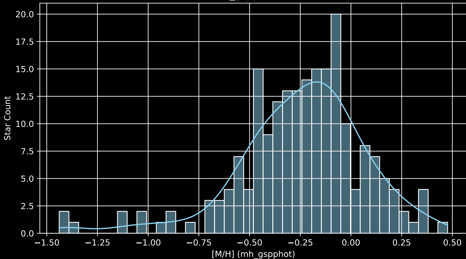
APOGEE DR17 Field: [237+44_MGA [M/H] (mh_gspphot) (n= 204)
