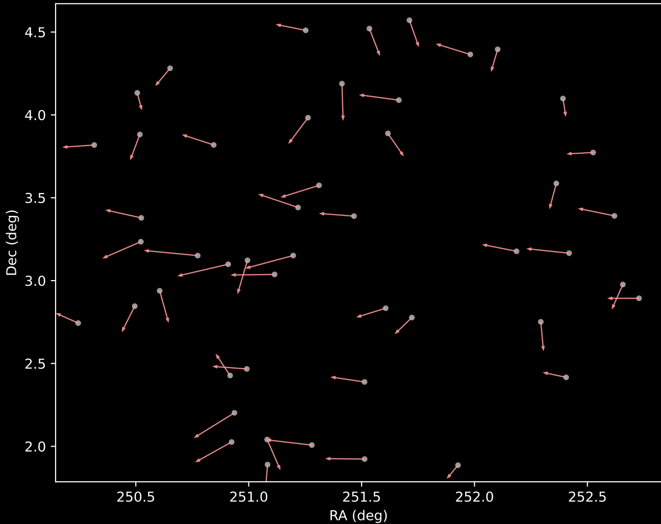
APOGEE DR17 Cluster 7 Proper Motion Vectors (n=49)
