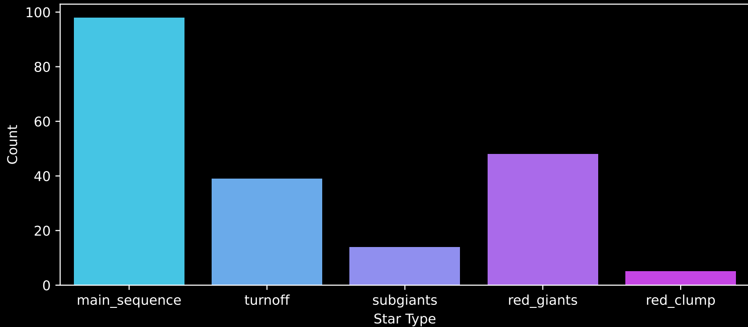
APOGEE DR17 Field: [237+44_MGA] Count plot of Star Type
